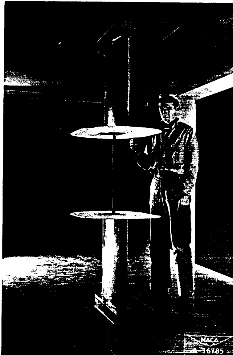
Figure 2.- Method of mounting 1-inch cylinders between end plates in the wind tunnel.
