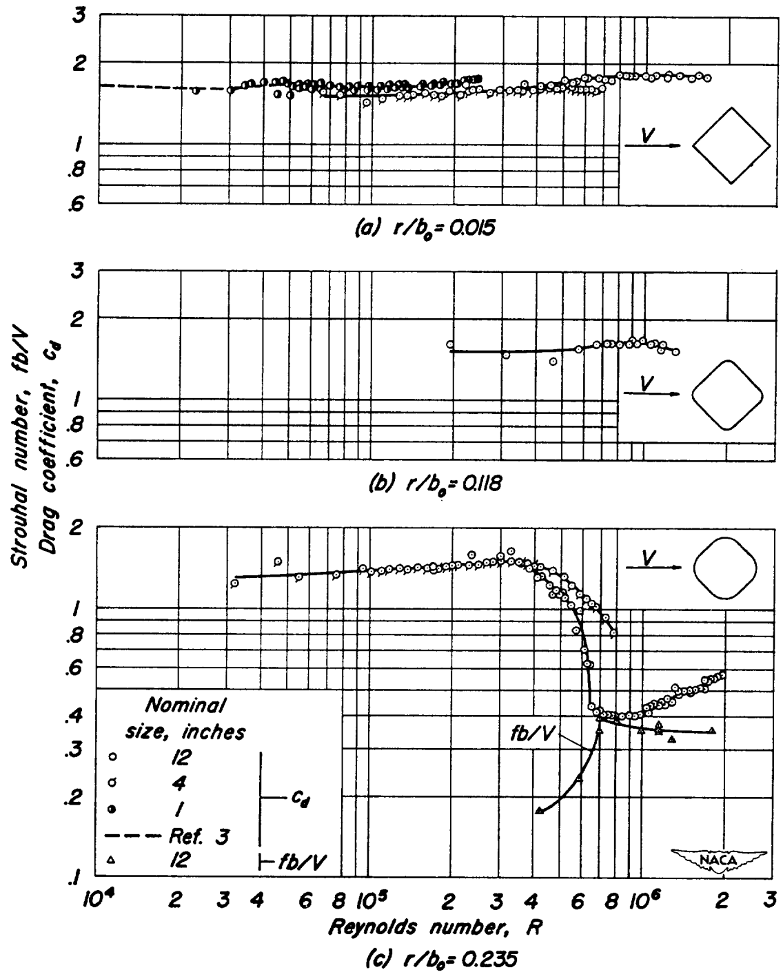
Figure 11.—Variation of drag coefficient and Strouhal number with Reynolds number for the 1:1 fineness ratio diamond cylinders.
