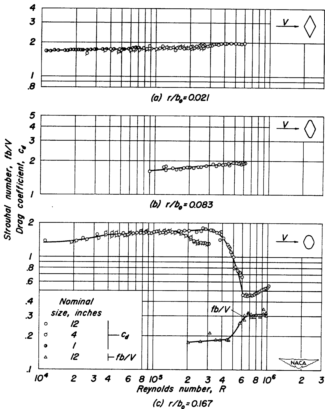
Figure 10.—Variation of drag coefficient and Strouhal number with Reynolds number for the 1:2 fineness ratio diamond cylinders.
