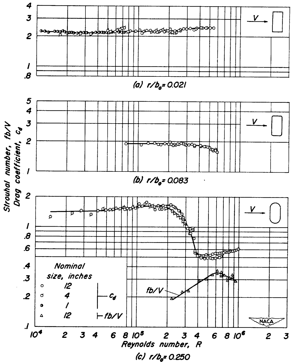
Figure 7.—Variation of drag coefficient and Strouhal number with Reynolds number for the 1:2 fineness ratio rectangular cylinders.
