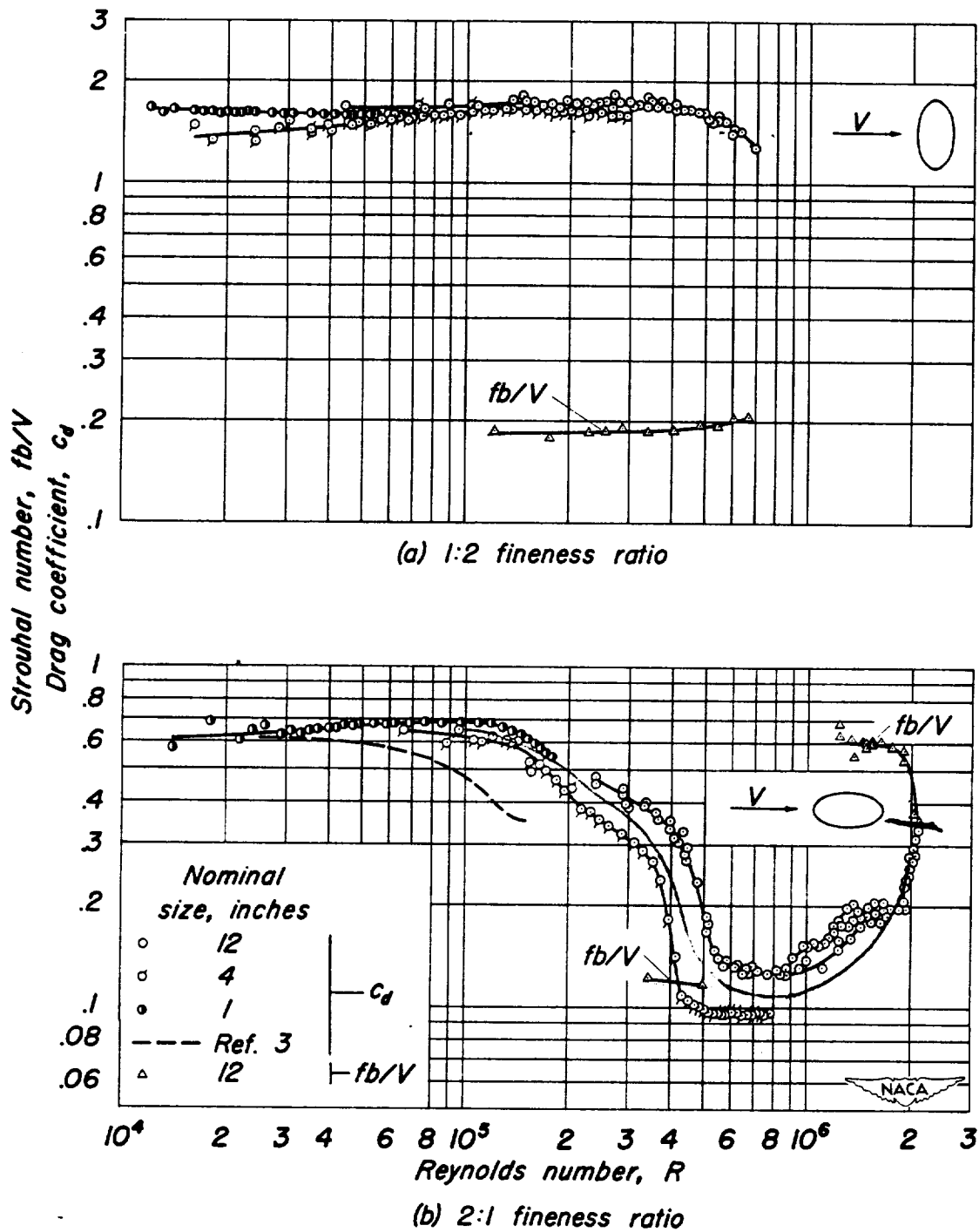
Figure 6.—Variation of drag coefficient and Strouhal number with Reynolds number for the elliptic cylinders.
